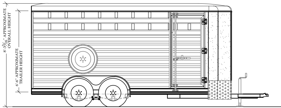
B CURB SIDE VIEW SCALE: 1/4" = 1'-0"
