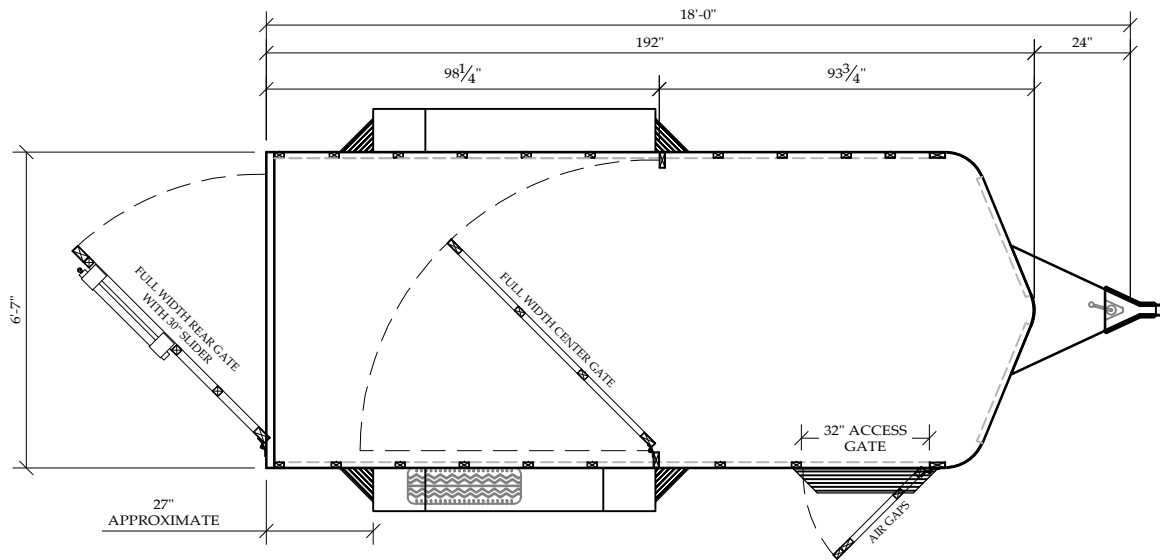
A TOP DOWN VIEW SCALE: 1/4" = 1'-0"
