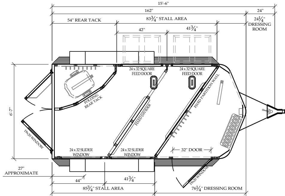
A TOP DOWN VIEW SCALE: 1/4" = 1'-0"
